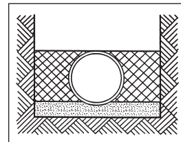
Type 4 Pipe bedded in sand, gravel, or crushed stone to depth of \frac{1}{8} pipe diameter, 4-in. minimum. Backfill compacted to top of pipe. (Approximately 80% Standard Proctor, AASHTO T-99.)§
